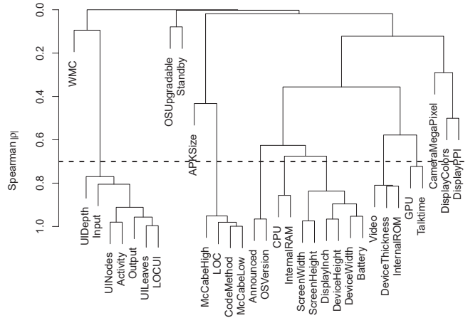
Fig. 6: Hierarchical clustering of app and device attributes according to the Spearman's |\rho|
